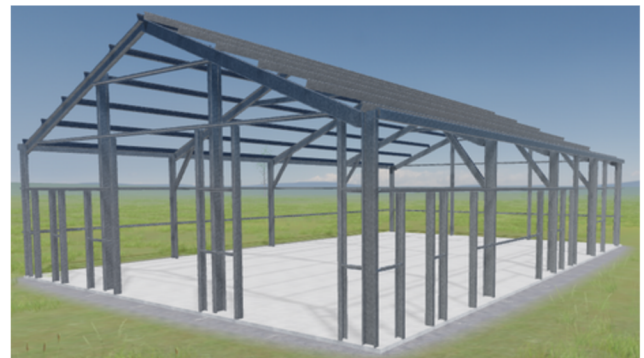
Panels removed showing the RAPID Steel cold formed structure only
